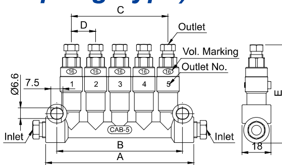
Dimensional Drawing of CAB-5-A-44444-AA
