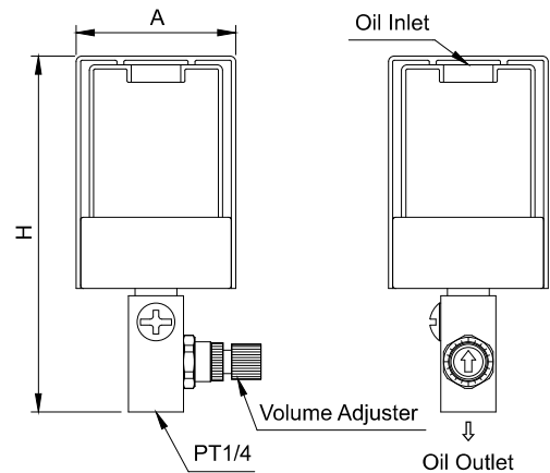
OP Dimensional Drawing
