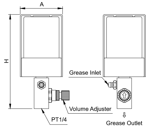
GP Dimensional Drawing
